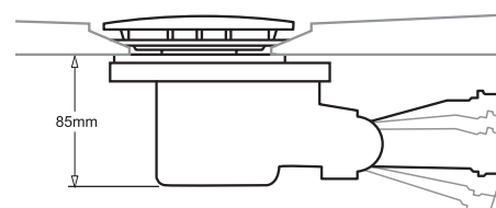
Diagram. a Matki Fastflow Shower Waste
