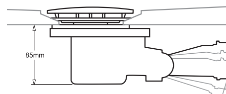
Diagram. a Matki Fastflow Shower Waste
